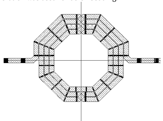
Figure 2 : Symmetric inductor layout
